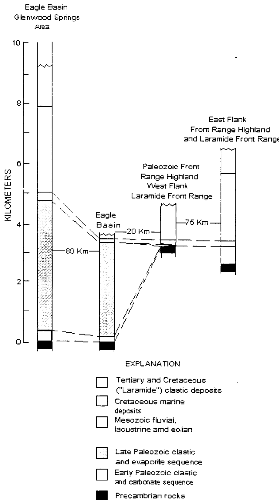
Figure 4. Comparison of generalized stratigraphic sections from the Denver basin across the Front Range Highland and into the Eagle basin along the field trip route. Sections correspond to those in Table 1.
